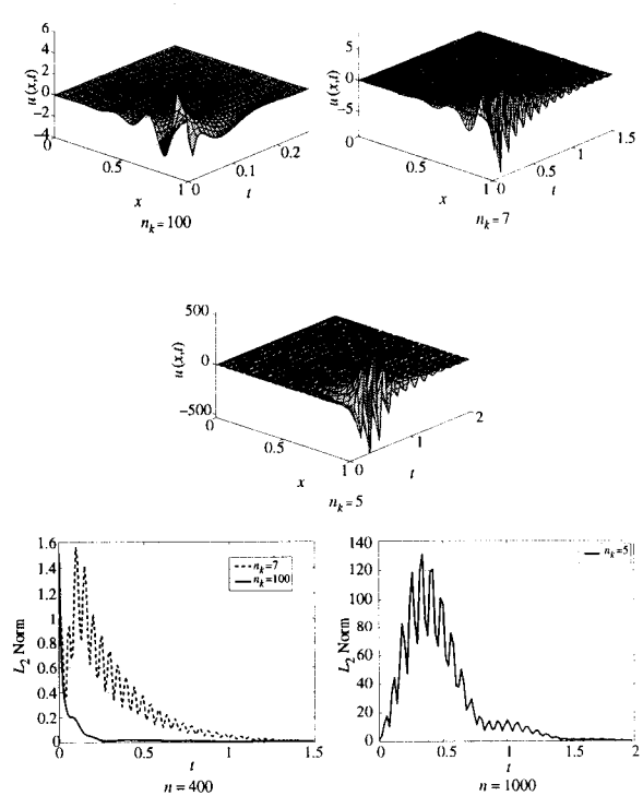
Fig. 8. Approximation of controlled system using reduced controllers.
