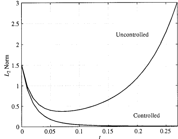
Fig. 7. Comparison of L_2 -norms.
