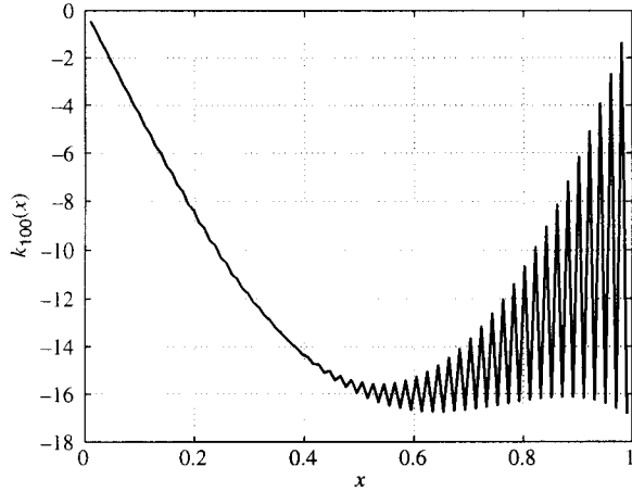
Fig. 2. Oscillation of the approximating kernel for n = 100 , \lambda = 17 , \varepsilon = 1 , c = 0 .
