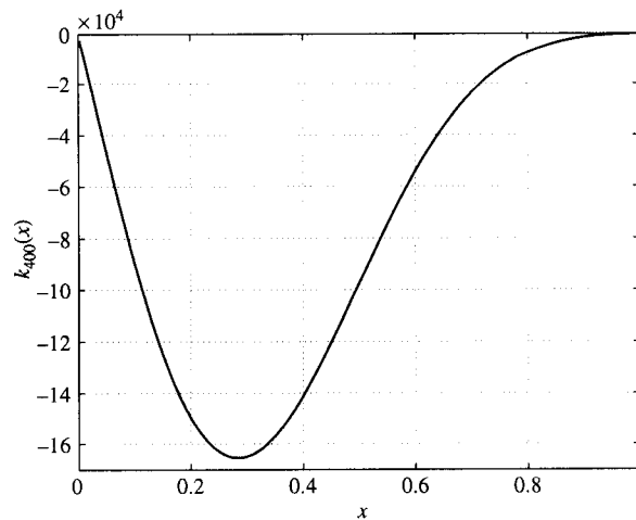
Fig. 4. Kernel function k_n(x) for n = 400 .
