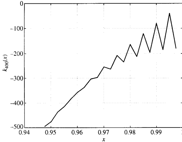
Fig. 5. Oscillation of the approximating kernel function.
