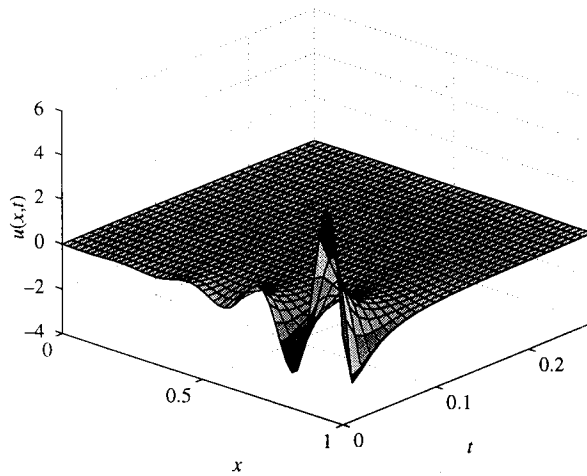
Fig. 6. Approximation of controlled system for n = 400 .
