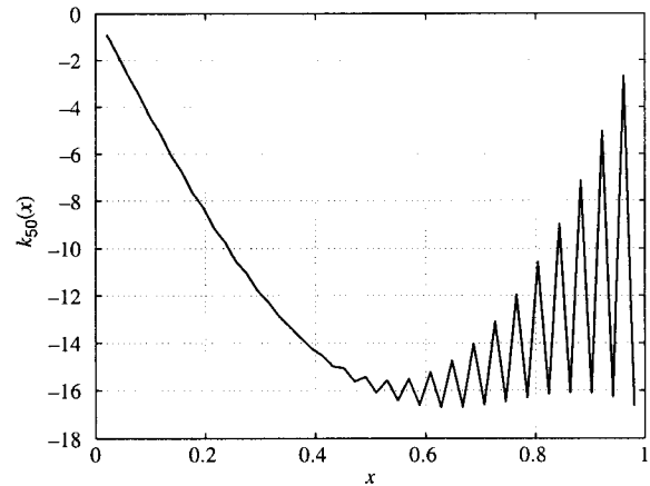
Fig. 1. Oscillation of the approximating kernel for n = 50 , \lambda = 17 , \varepsilon = 1 , c = 0 .
