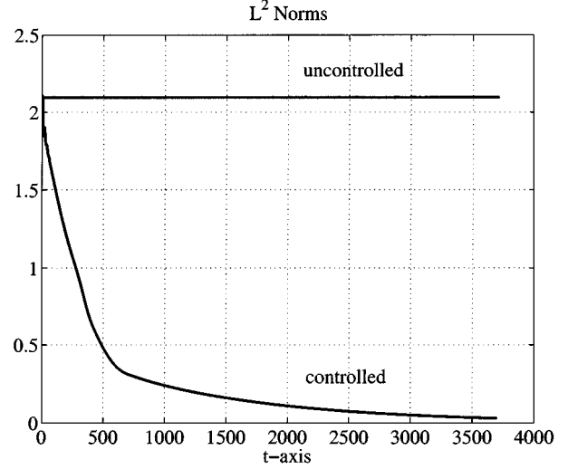
Fig. 3. Energy comparison.
