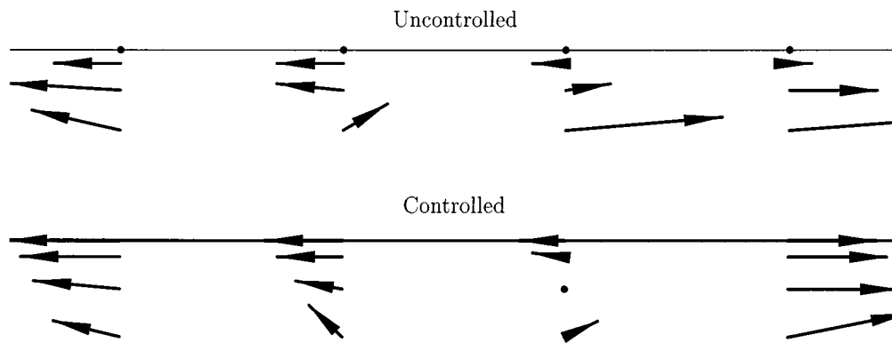
Fig. 6. Velocity field in a rectangle of dimension 0.393 \times 0.012 zoomed out of a channel of dimension 4\pi \times 2 , at time t = 120 . The control (thick arrows) acts both downstream and upstream . The control maintains the value of shear near the desired (laminar) steady-state value.
