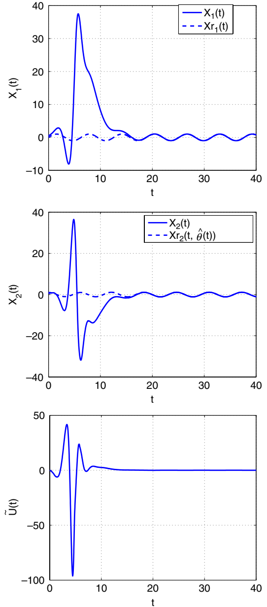
Fig. 1. The system response of the system (1)–(2) with the reference trajectory (20)–(21) for D = 1 , \theta = 0.5 , \hat{\theta}(0) = 0 and \hat{D}(0) = 0 .
