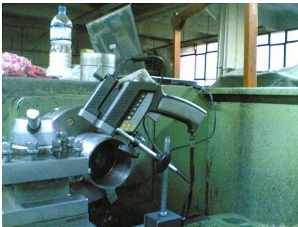
Fig. 8 Infrared camera installation on the lathe
