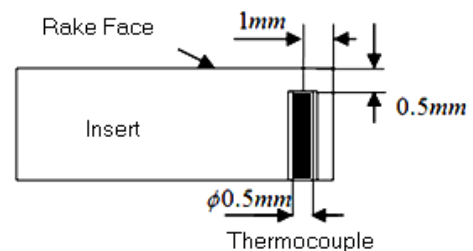
Fig. 2 The schematic outline of insert
