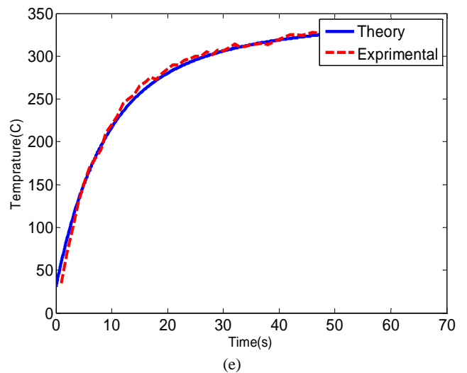
Fig. 6 F Tool temperature vs. Time in (a) V=131 mm/s, (b) V=185 mm/s, (c) V=263 mm/s (d) V=528 mm/s and (e) V=733 mm/s
